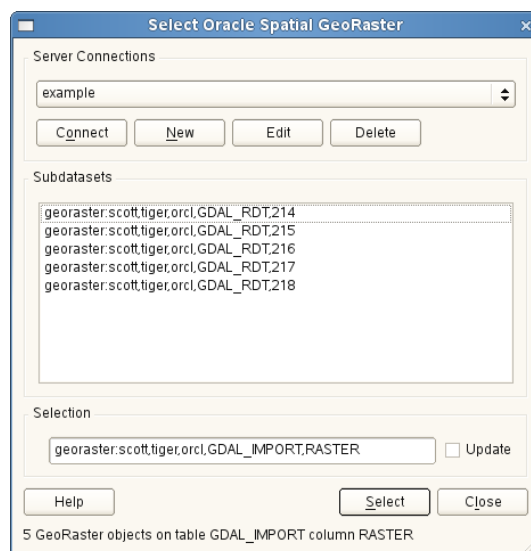
Figure 18.26: Select Oracle GeoRaster dialog
