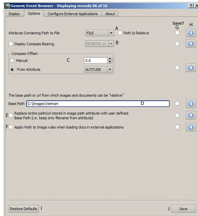
Figure 18.10: The eVis Options window
