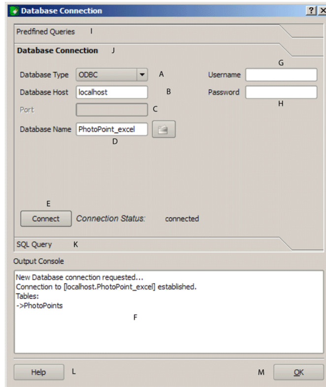
Figure 18.12: The eVis Database connection window
