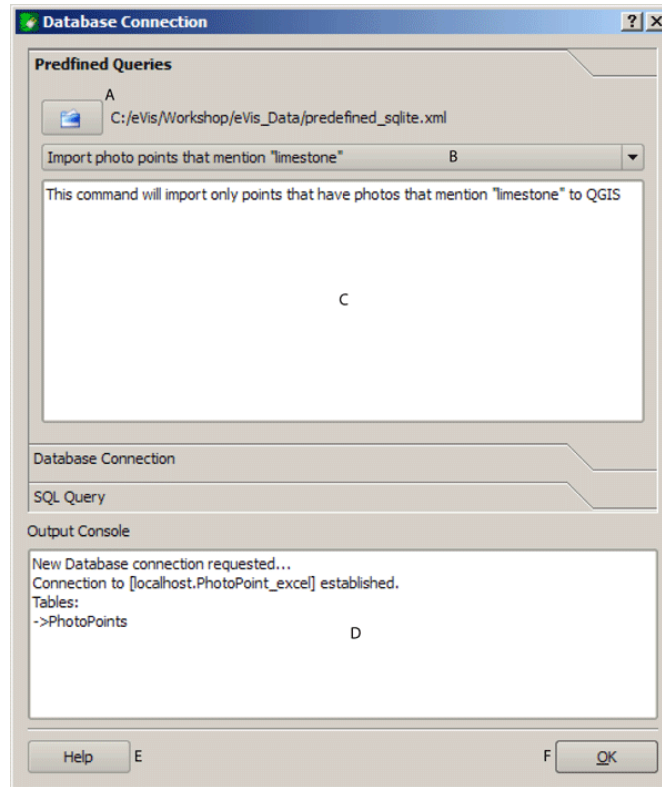
Figure 18.14: The eVis Predefined queries tab
